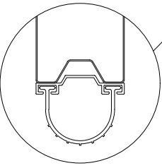
Bottom Seal Detail TPE astragal in aluminum retainer
