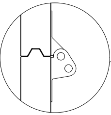
Hinge Detail Graduated end hinges ≥ 16'-3" wide = double end hinges minimum 14 gauge
