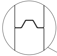
Joint Detail Tongue and groove design with flexible gasket between sections
